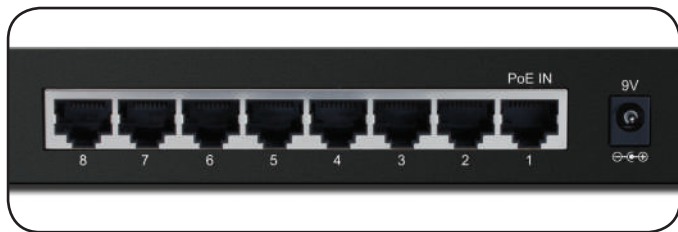
AGS-1008M Rear Panel View
