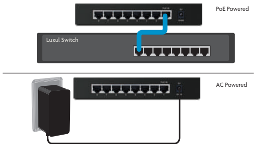
Powering the AGS-1008M by AC or PoE
