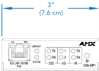
EXB-MP1 (Front View)
