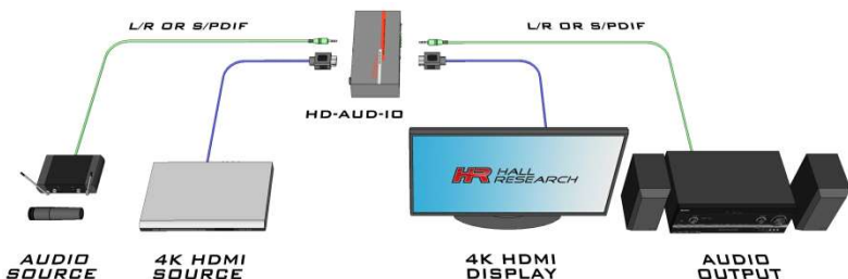
Typical Connection Diagram
