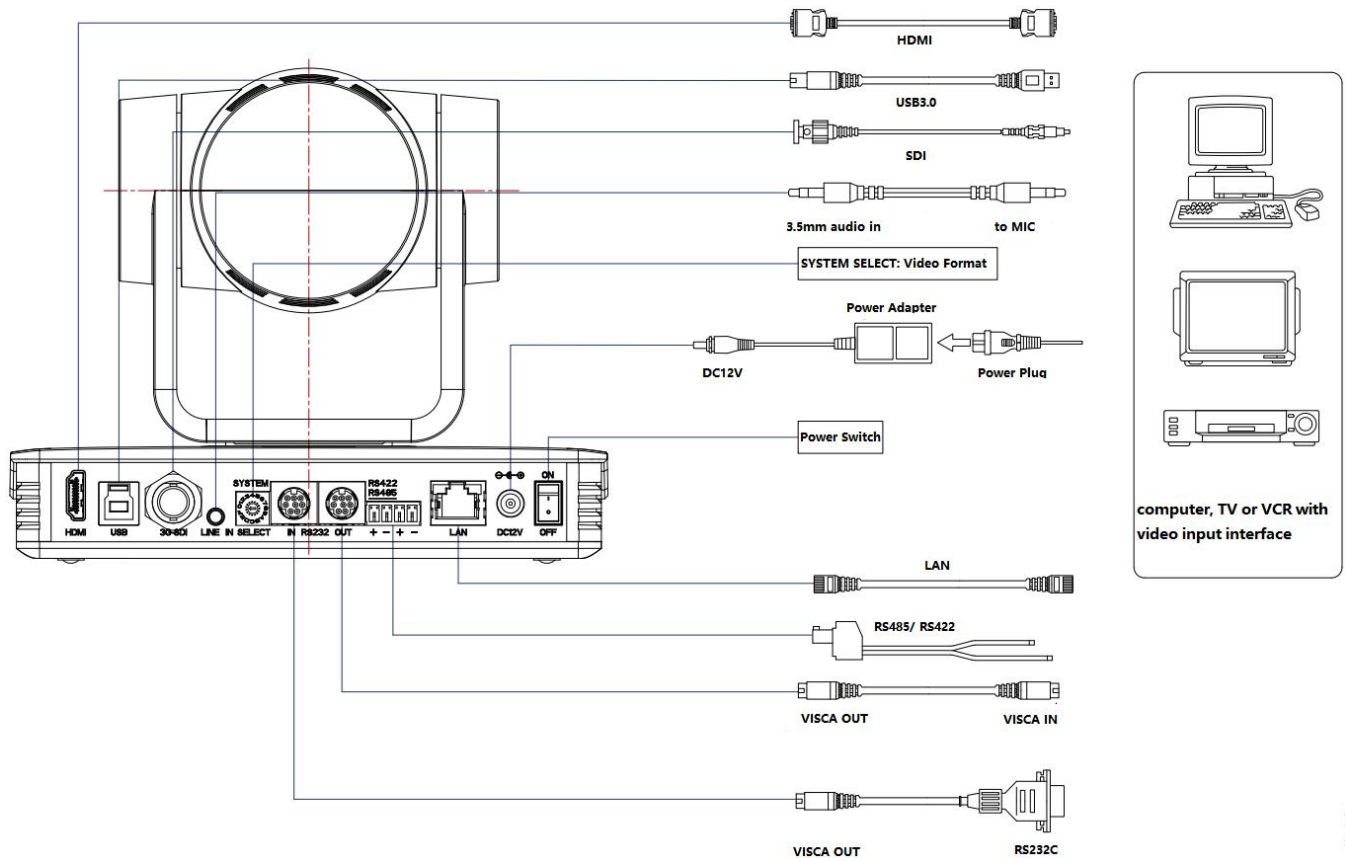
Figure 1.3 Wiring Diagram
