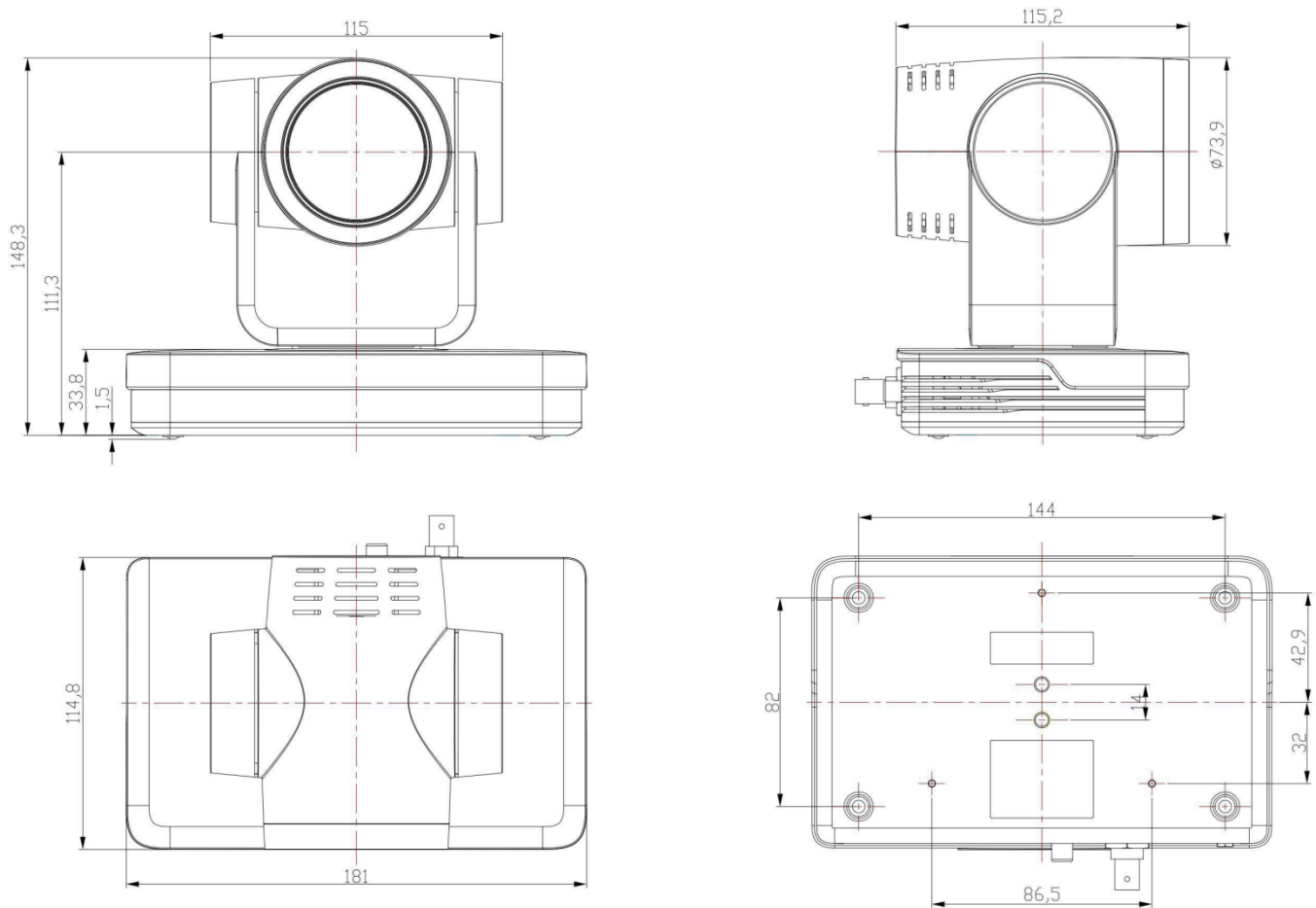
Figure 2.2 Product Dimensions
