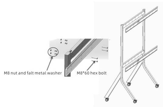
For 120/150-inch
