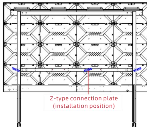
For 120/150-inch
