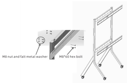
For 138/165-inch
