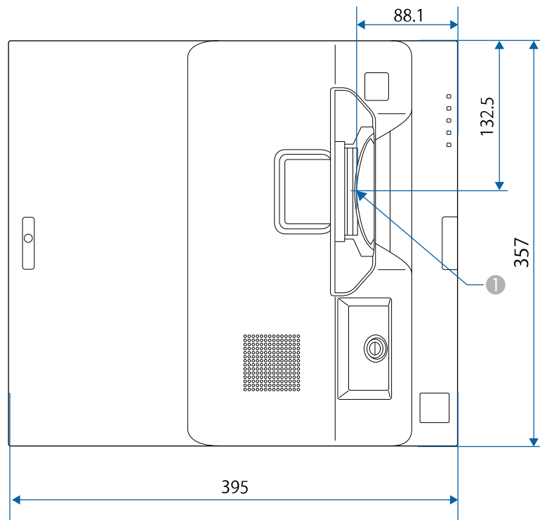
① Center of the projection lens
