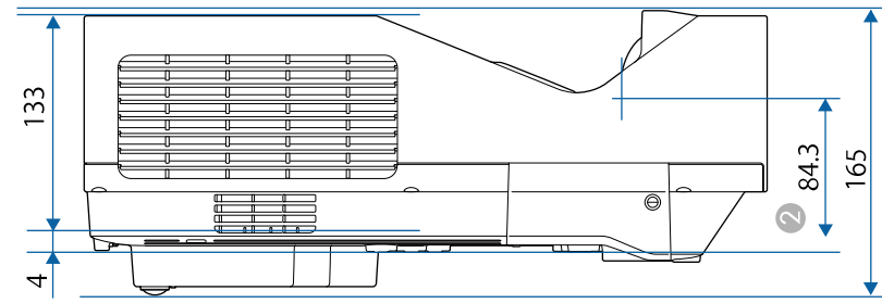
② Distance from the center of the projection lens to the ceiling mount fixing points
